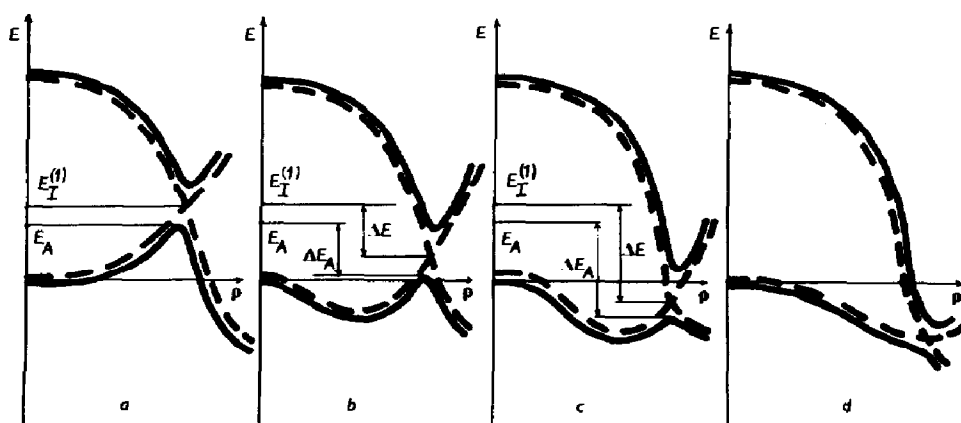
Fig. 11. The cross-section of the lowest adiabatic potential surface along the E coordinate without (a), and with weak \Delta E_A < E_A (b), sufficiently strong \Delta E_A > E_A (c), and very strong (d) pseudo-Jahn-Teller effect in the cases of weak (broken curves) and strong (solid curves) interaction with the decay term E_3 .
