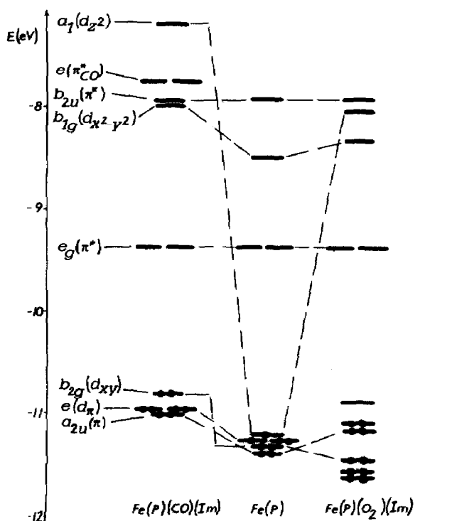
Fig. 6. Energy levels for the highest occupied and lowest unoccupied MO of ferroporphyrin complexes with [47] and without [31] axial ligands.
