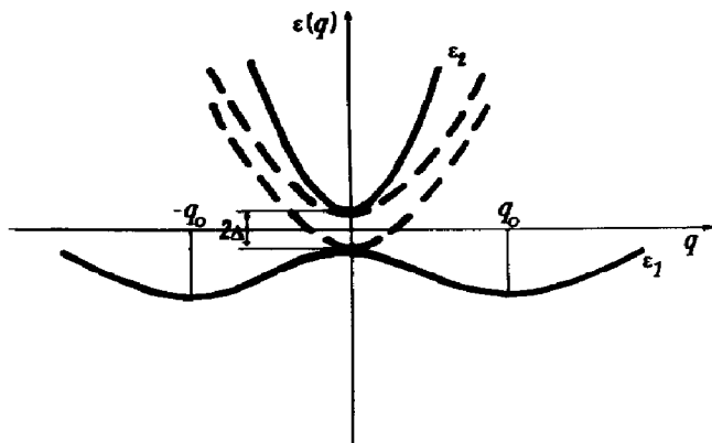
Fig. 1. The shape of the adiabatic potential sheets with (solid lines) and without (broken lines) the pseudo-Jahn-Teller effect for two non-degenerate mixing terms.
